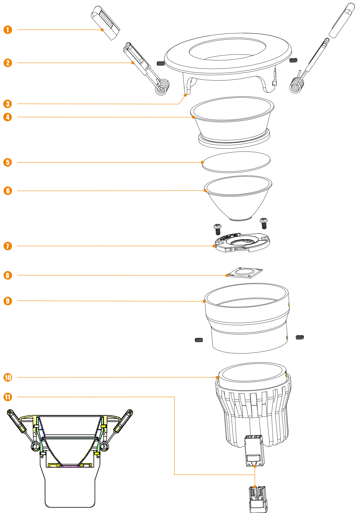
LED DOWNLIGHT DH
