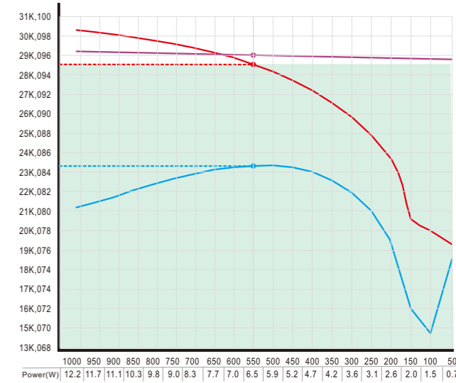
— CRI — CCT — light efficiency — DH1295S CCT dim range 31K, 100=3100K, CRI 100 and 100LM/W 1000=1000LM 950=950LM 900=900LM.....
